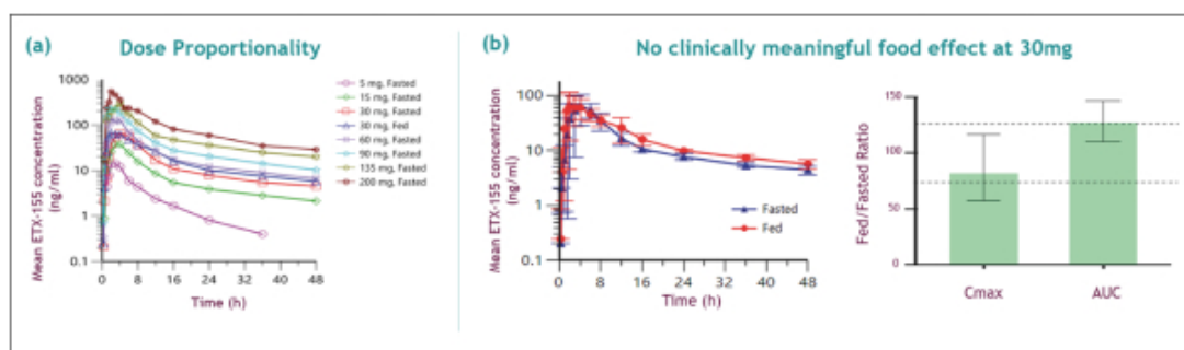
Figure 17. ETX-155 Pharmacokinetics from SAD. (a) ETX-155 showed well-behaved pharmacokinetics, with dose proportional increase in C max and AUC across a 5 to 200 mg dose range, with small/moderate inter-subject variability (CV≤30%). (b) Pharmacokinetics and fed/fasted ratio for ETX-155 30 mg fed and fasted cohort. ETX-155 did not demonstrate any clinically meaningful differences in C max or AUC upon administration in a fed or fasted state, with a C max fed/fasted ratio of 0.89 and an AUC fed/fasted ratio of 1.23, confirming a lack of food effect.
